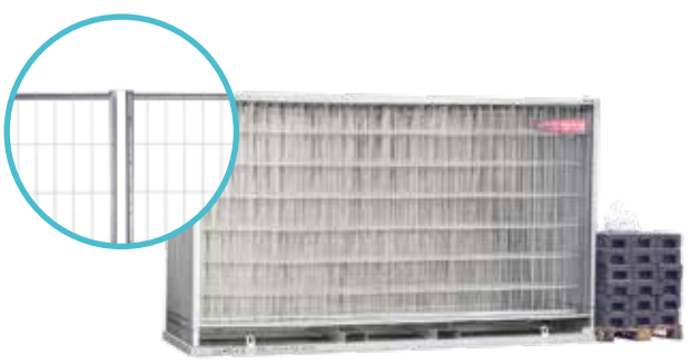
Mobile Secure Original Artnr. KIT 105M 01 1st Transportpall 30st Mobile Secure 3,5m paneler 30st Demex 20kg fundament 30st kopplingsklammer 0,5kg
